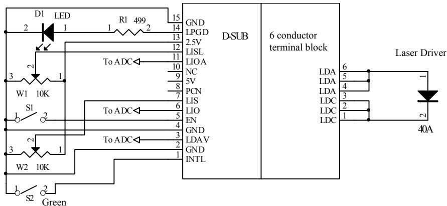
Figure 4. A Typical Application Schematic
