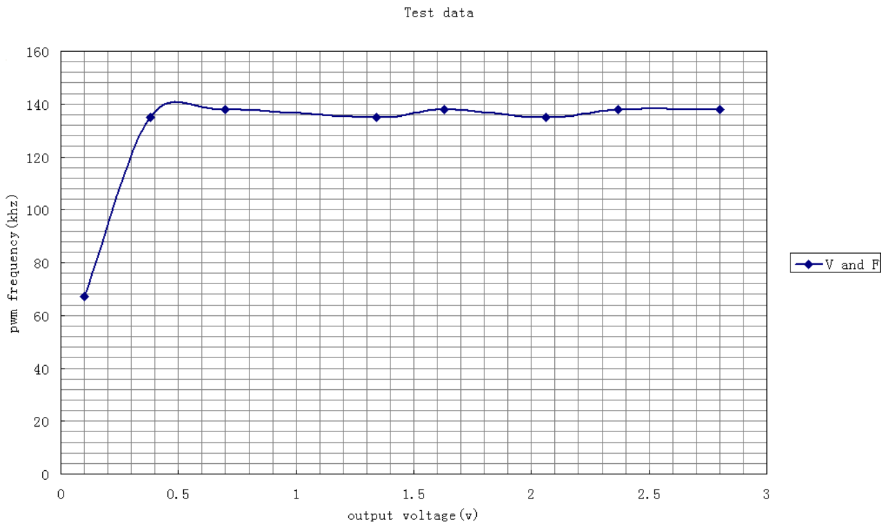
Figure 9. Output Voltage vs. PWM Frequency
