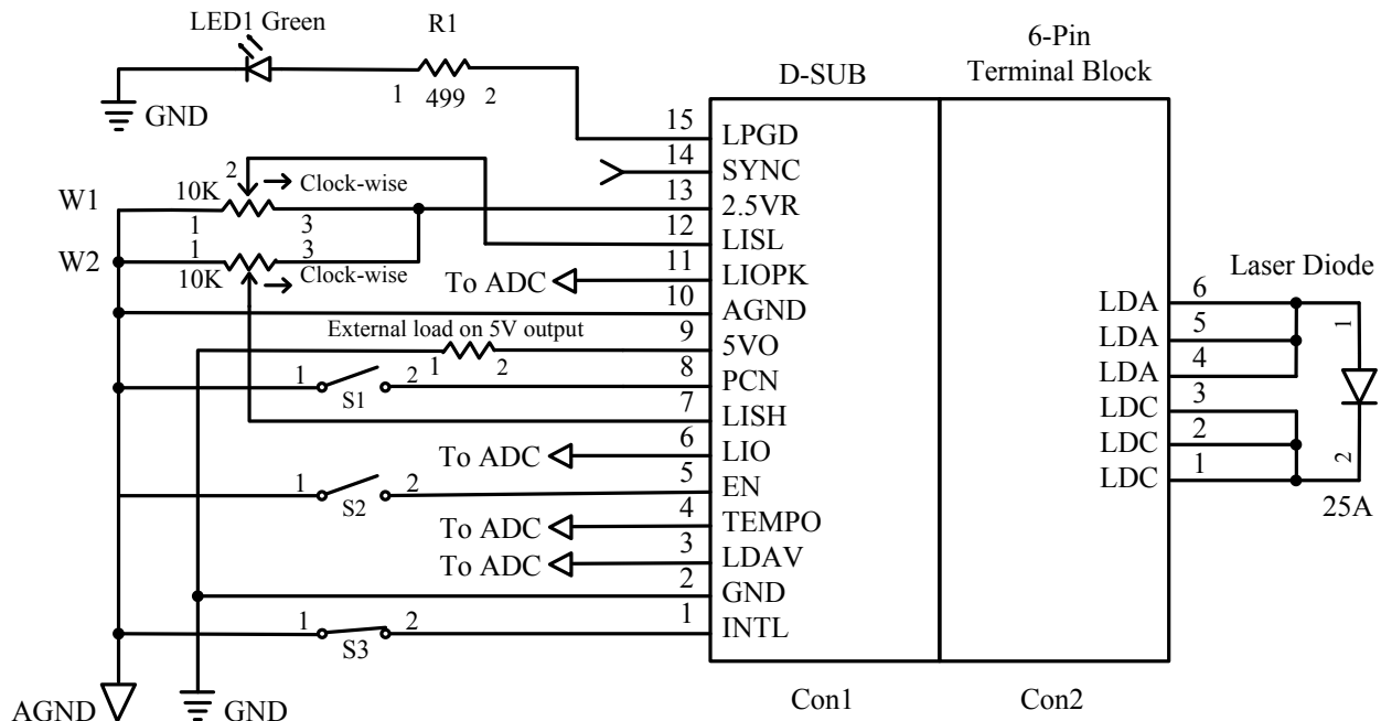
Figure 3. A Typical Application Schematic
