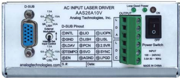
Figure 1. Front View of the AAS26A10V
