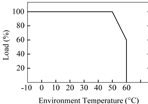
Figure 25. Derating Curve
