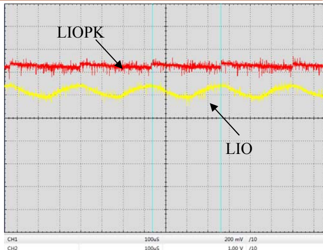
Figure 18. Digital Modulation Response at LIOPK & LIO Pin (f=3kHz)
