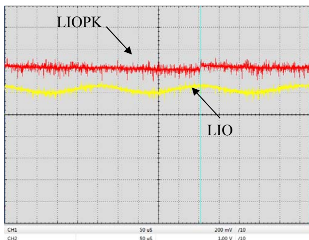
Figure 20. Digital Modulation Response at LIOPK & LIO Pin (f=4kHz)
