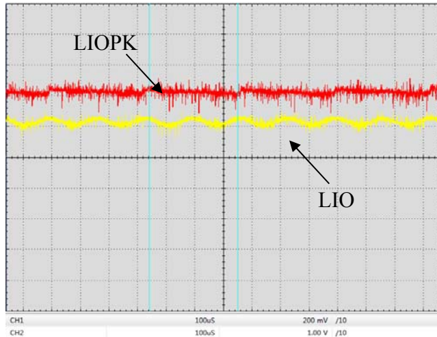
Figure 24. Digital Modulation Response at LIOPK & LIO Pin (f=6kHz)
