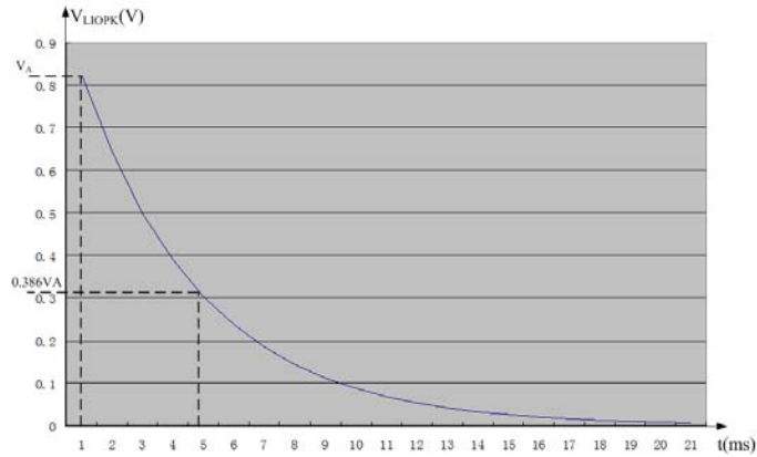
Figure 5. LIOPK's Mathematic Model
