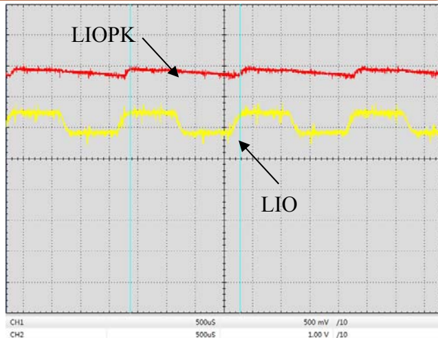
Figure 12. Digital Modulation Response at LIOPK & LIO Pin (f=500Hz)
