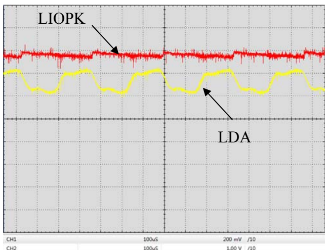
Figure 17. Digital Modulation Response at LIOPK & LDA Pin (f=3kHz)
