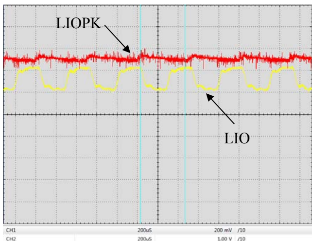
Figure 16. Digital Modulation Response at LIOPK & LIO Pin (f=2kHz)
