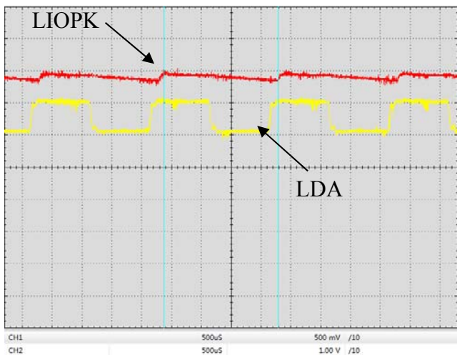
Figure 11. Digital Modulation Response at LIOPK & LDA Pin (f=500Hz)
