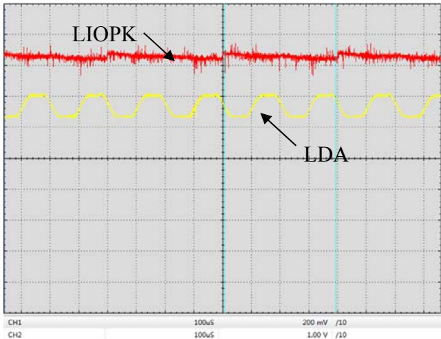
Figure 21. Digital Modulation Response at LIOPK & LDA Pin (f=5kHz)
