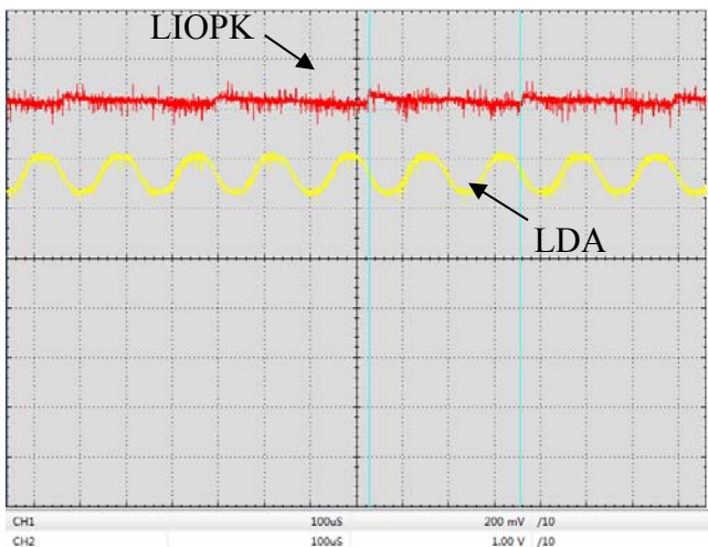
Figure 23. Digital Modulation Response at LIOPK & LDA Pin (f=6kHz)
