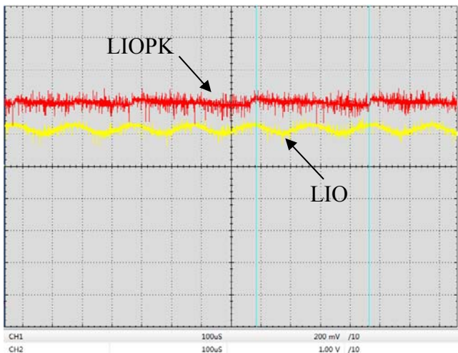
Figure 22. Digital Modulation Response at LIOPK & LIO Pin (f=5kHz)
