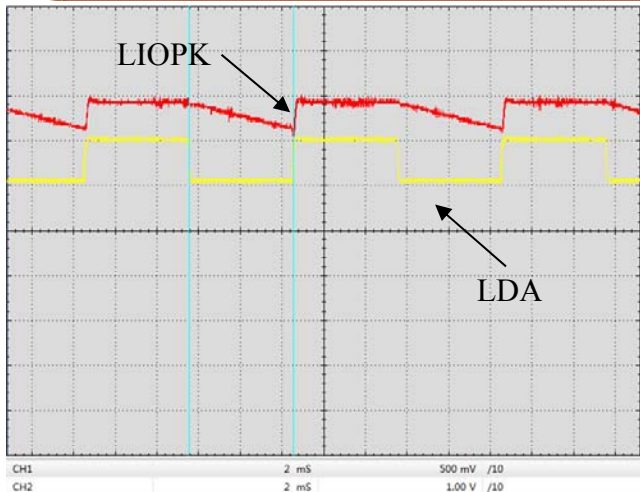
Figure 9. Digital Modulation Response at LIOPK & LDA Pin (f=100Hz)
