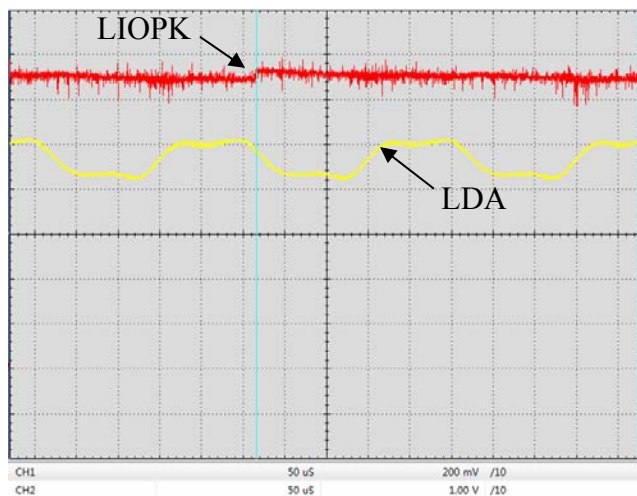
Figure 19. Digital Modulation Response at LIOPK & LDA Pin (f=4kHz)
