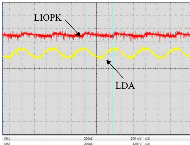
Figure 15. Digital Modulation Response at LIOPK & LDA Pin (f=2kHz)
