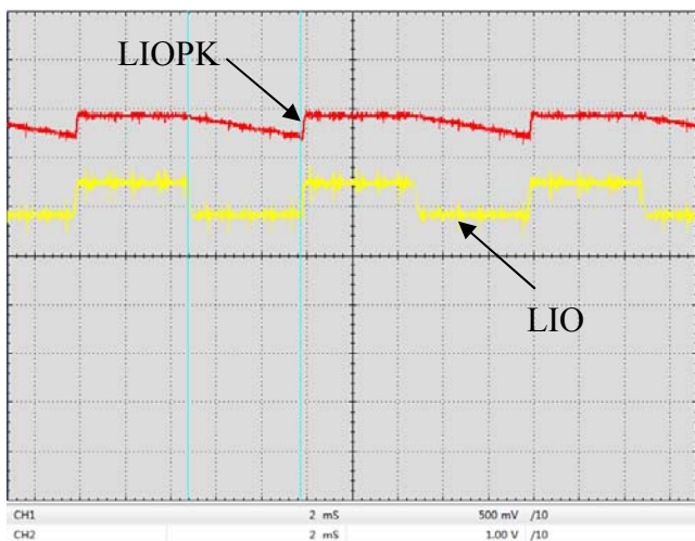
Figure 10. Digital Modulation Response at LIOPK & LIO Pin (f=100Hz)
