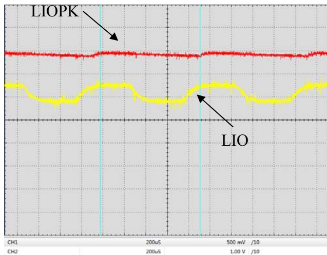
Figure 14. Digital Modulation Response at LIOPK & LIO Pin (f=1kHz)
