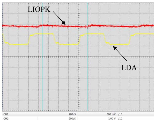
Figure 13. Digital Modulation Response at LIOPK & LDA Pin (f=1kHz)
