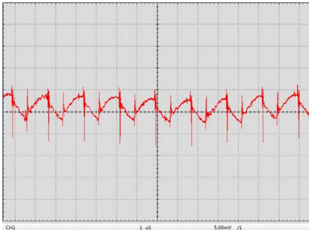
Figure 27. Noise Waveform at LDA Pin
