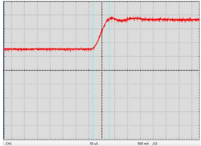
Figure 6. Digital Modulation Response at LDA Pin
