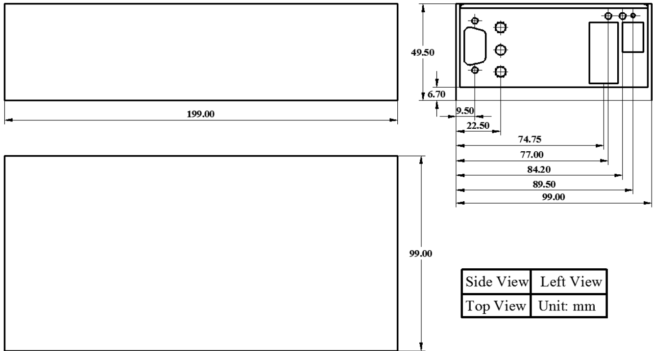
Figure 29. Mechanical Dimensions
