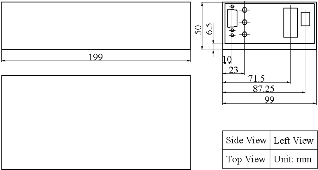
Figure 9. Mechanical Dimensions
