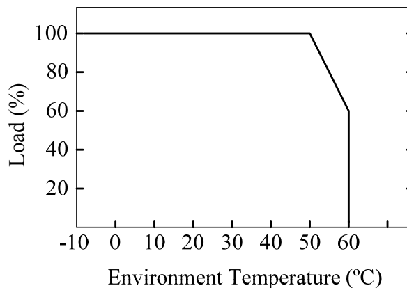
Figure 16. Derating Curve
